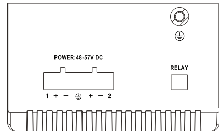
Figure 3-2 AIS4001P side panel
