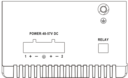
Figure 3-2 AIS2004P side panel
