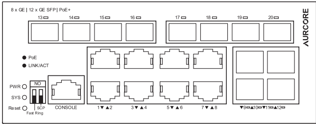
Figure 2-1 Switch front panel diagram
