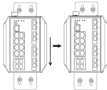
Schematic diagram of wall mounted installation of industrial machine
