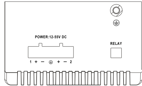
Figure 3-2 AIS2004 side panel
