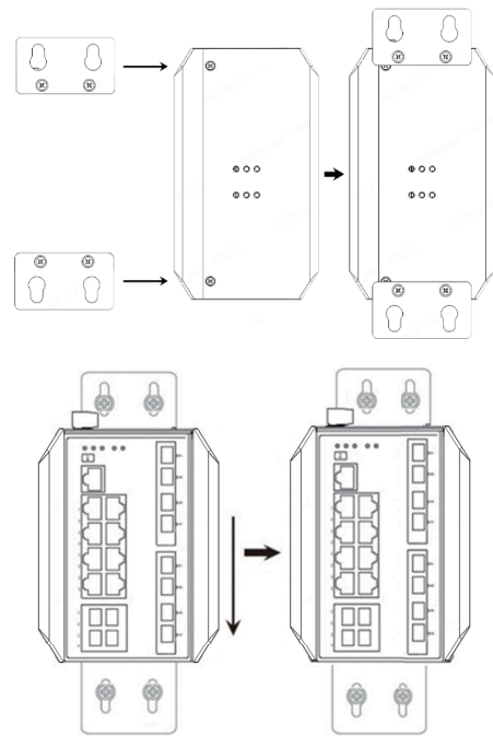
Schematic diagram of wall mounted installation of industrial machine
