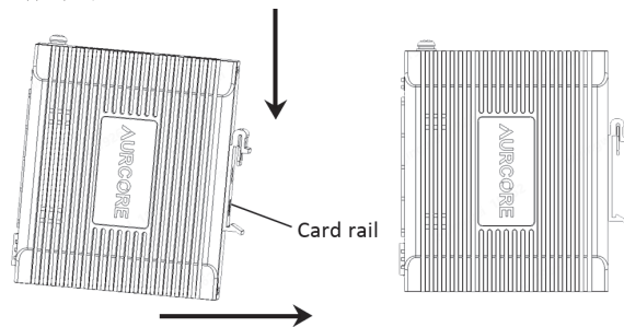
Figure 4-1 Schematic diagram of industrial machine guide rail installation
