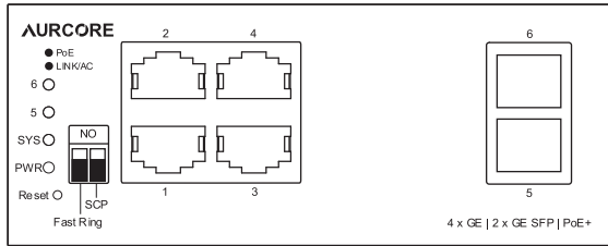
Figure 3-1 Front panel of the 4-Port Gigabit+2G SFP Switch
