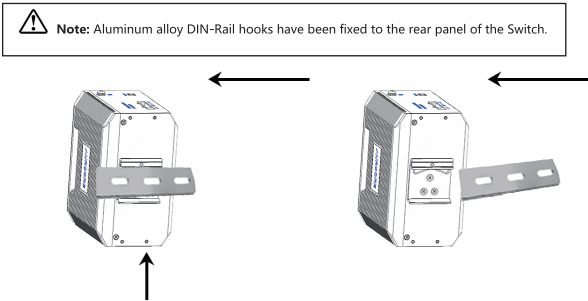
Figure 4-2 Schematic diagram of industrial machine guide rail disassembly
