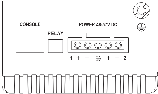
Figure 3-2 Side panel of a 4-Port Gigabit+2G SFP Switch
