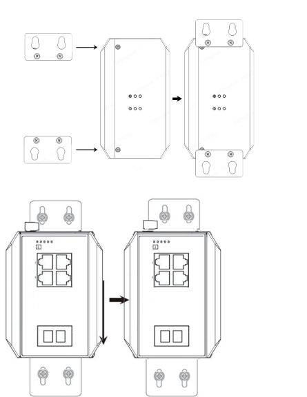
Schematic diagram of wall mounted installation of industrial machine
