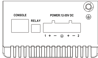
Figure 3-2 Side panel of the 4-Port Gigabit +2G SFP Switch
