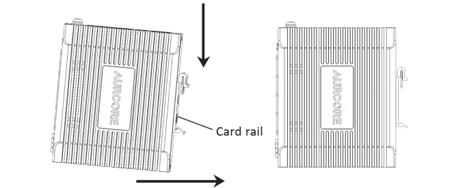
Figure 4-1 Schematic diagram of industrial machine guide rail installation Note: Aluminum alloy DIN-Rail hooks have been fixed to the rear panel of the Switch.
