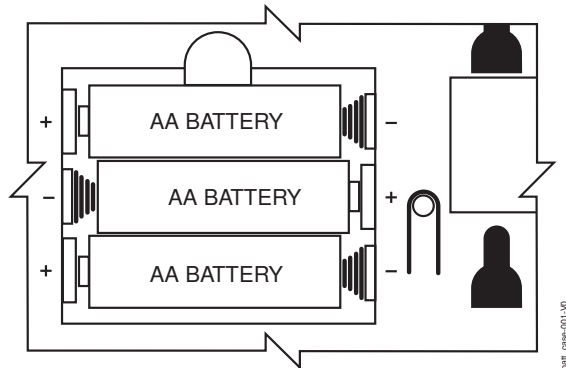
Battery Compartment
